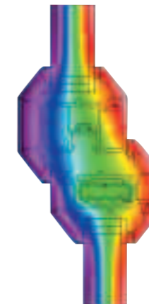
Thermal transfer through Liniar 'A Rated' sash/transom
