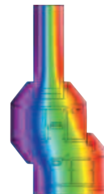
Thermal transfer through Liniar 'A Rated' sash/outer frame
